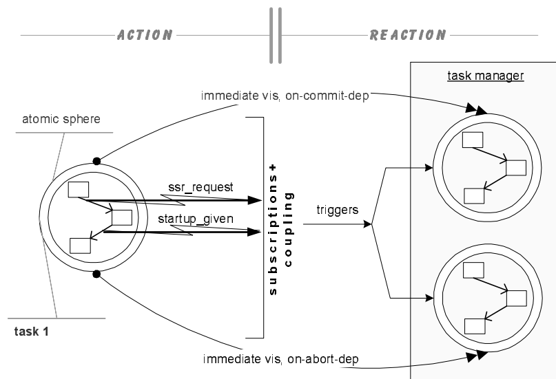
Figure 1 Event-based process enactment
