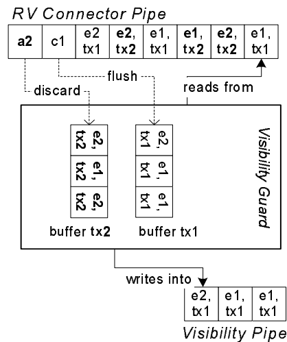
Figure 7 Visibility guard
