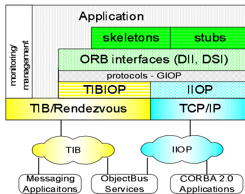
Figure 4 ObjectBus architecture
