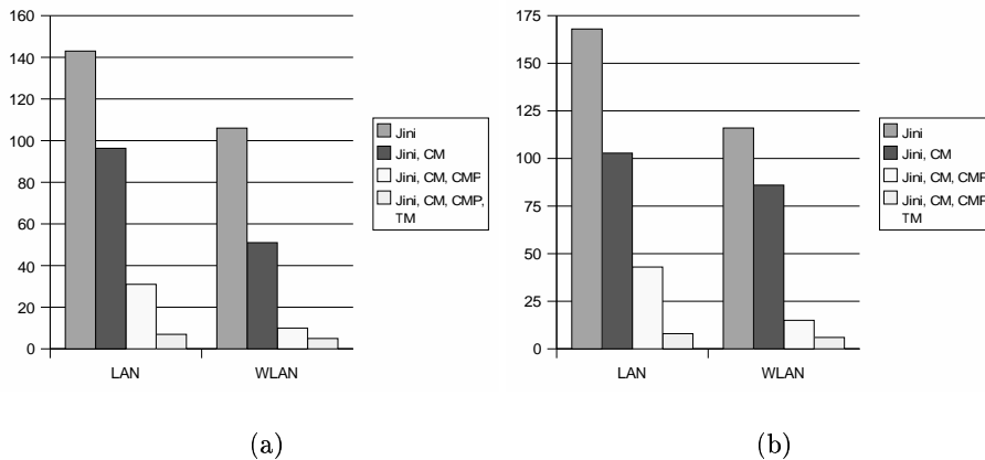
Fig. 9. (a) Comparative throughputs (inv/s) between the fixed and mobile infrastructure for the (1,1) configuration and (b) Comparative throughputs (inv/s) for the (2,1) configuration.
