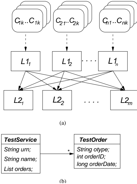
Fig. 5. (a) Three level configuration used for measurements and (b) The local data structure present at each service.
