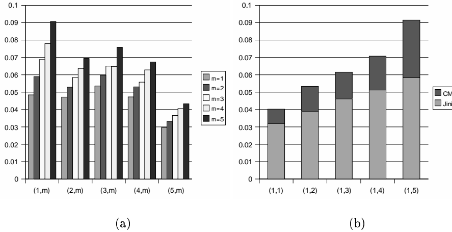
Fig. 6. (a) Response times (s) with no extensions.(b) Response times (s) for the (1,m) measurements, with CM.
