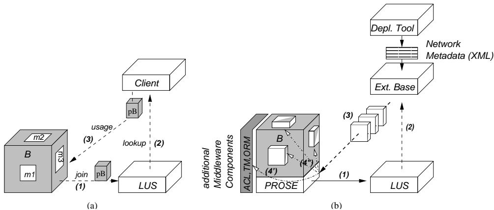
Fig. 2. (a) Typical interactions in Jini and (b) Run-time adaptation of application through a Jini interface.
