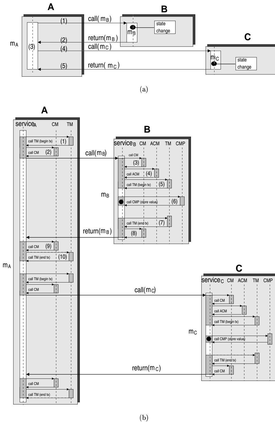
Fig. 3. (a) Initial control flow and (b) Control flow after extensions have been added.
