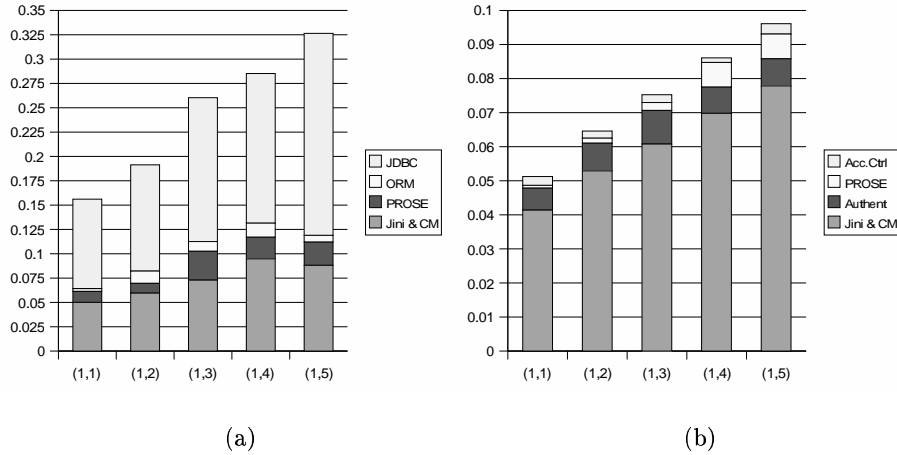
Fig. 8. (a) Response times (s) for the (1,m) measurements (with the CM and CMP extensions) and (b) Response times (s) for the (1,m) measurements (with the CM and ACM extensions).
